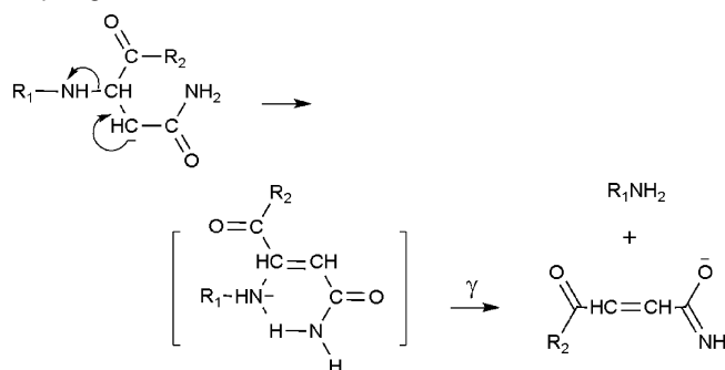
Scheme 6. \gamma Backbone Cleavage of Anionic Peptides at an Asparagine Residue 47
