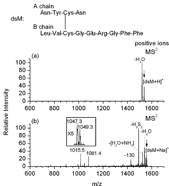
Figure 9. (a) MS^2 spectrum of singly charged protonated peptic digest fragment from insulin, NYCN/LVCGERGFF, at m/z 1537.5. (b) MS^2 spectrum of singly charged monosodiated peptic digest fragment from insulin, NYCN/LVCGERGFF, at m/z 1559.5, showing a major product involving elimination of H_2S_2 and four minor products from disulfide bond cleavages. Arrows indicate the ion peaks being isolated and collisionally activated.
