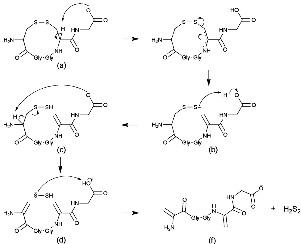
Scheme 4. Dissociation Mechanisms of Anionic Peptide CGGCG with Intramolecular Disulfide Bond via Enolization at Cys Backbone Proposed by Bilusich et al. 15 a
