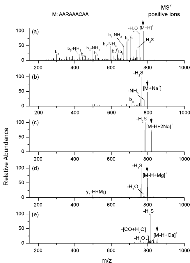
Figure 3. CID spectra of singly charged (a) protonated AARAAACAA, (b) monosodiated AARAAACAA, (c) disodiated AARAAACAA, (d) monomagnesium AARAAACAA, and (e) monocalcium AARAAACAA. Arrows indicate the ion peaks being isolated and collisionally activated.
