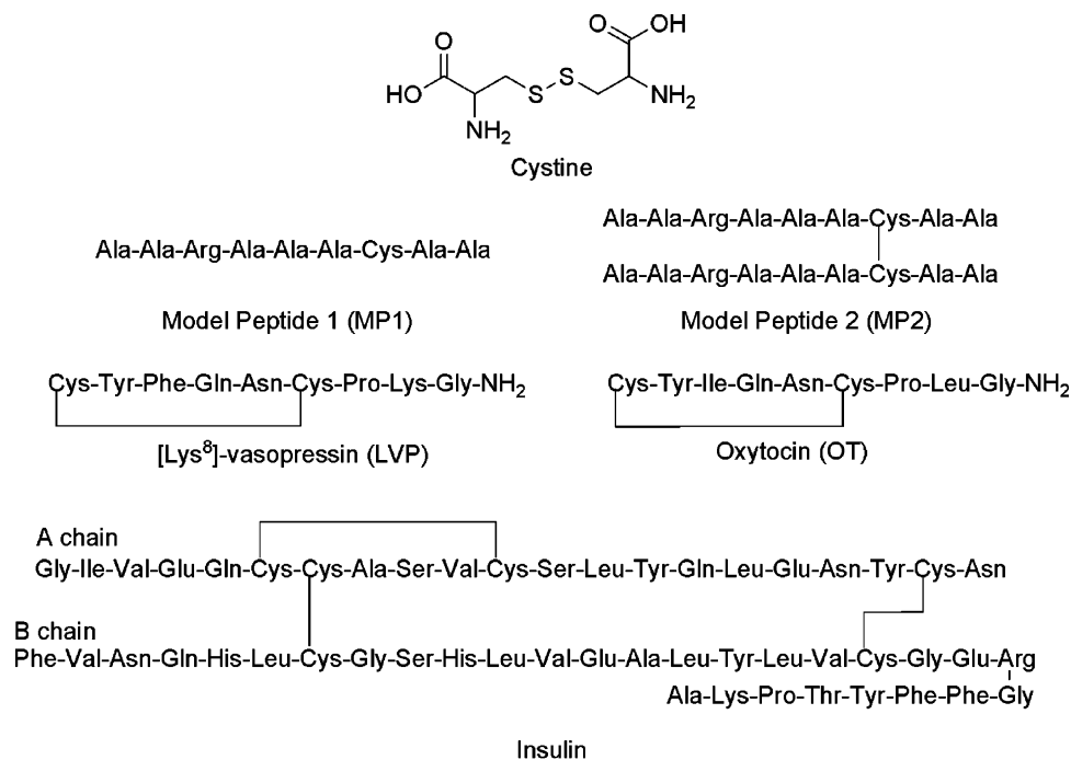
Figure 1. Structures of cystine, model peptides, nonapeptide hormones, and insulin examined in this study.
