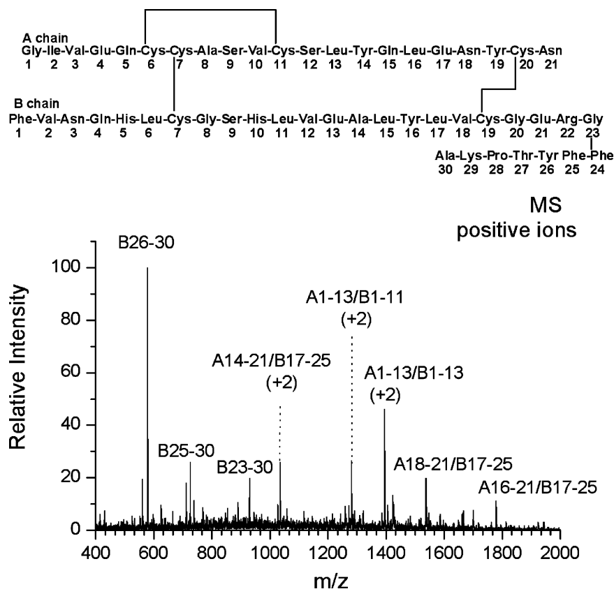
Figure 8. ESI-MS of pepsin digest of insulin in positive mode. Structure of insulin is shown with amino acid numbering of the two chains.
