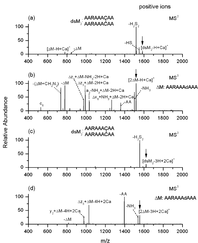
Figure 6. (a) MS 2 spectrum of singly charged monocalcium complex of disulfide linked AARAAACAA dimer showing a major product from elimination of H 2 S 2 and three minor products from H 2 S elimination and disulfide bond cleavages. (b) MS 3 spectrum of the major product from (a). (c) MS 2 spectrum of singly charged dicalcium complex of disulfide linked AARAAACAA dimer showing an exclusive product from elimination of H 2 S 2 . (d) MS 3 spectrum of the product from (c). Arrows indicate the ion peaks being isolated and collisionally activated.
