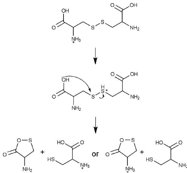
Scheme 3. A Charge Directed Neighboring Group Mechanism of Protonated Cystine for the Cleavage of S–S Bond Proposed by Lioe and O’Hair 12
