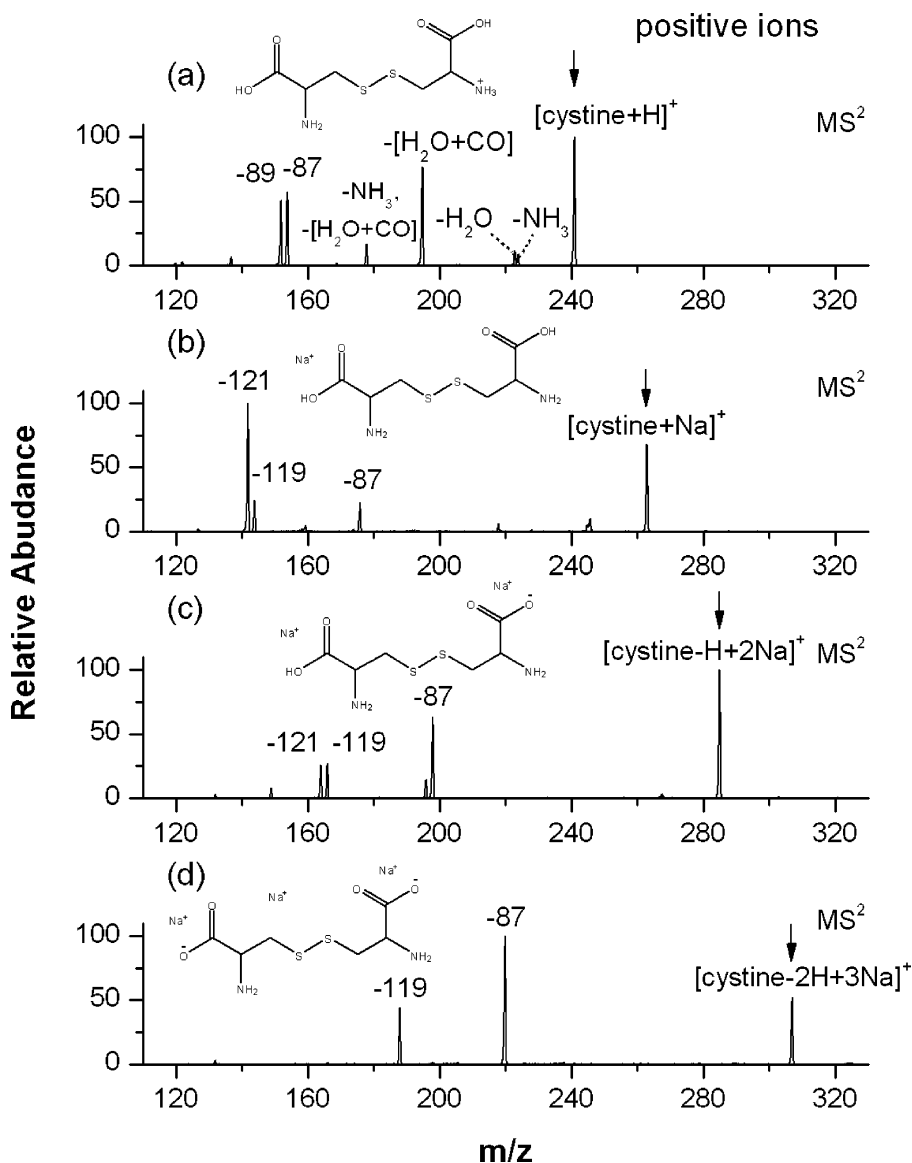
Figure 2. CID spectra of (a) protonated cystine, (b) singly sodiated cystine, (c) doubly sodiated cystine, and (d) triply sodiated cystine cations. Arrows indicate the ion peaks being isolated and collisionally activated.
