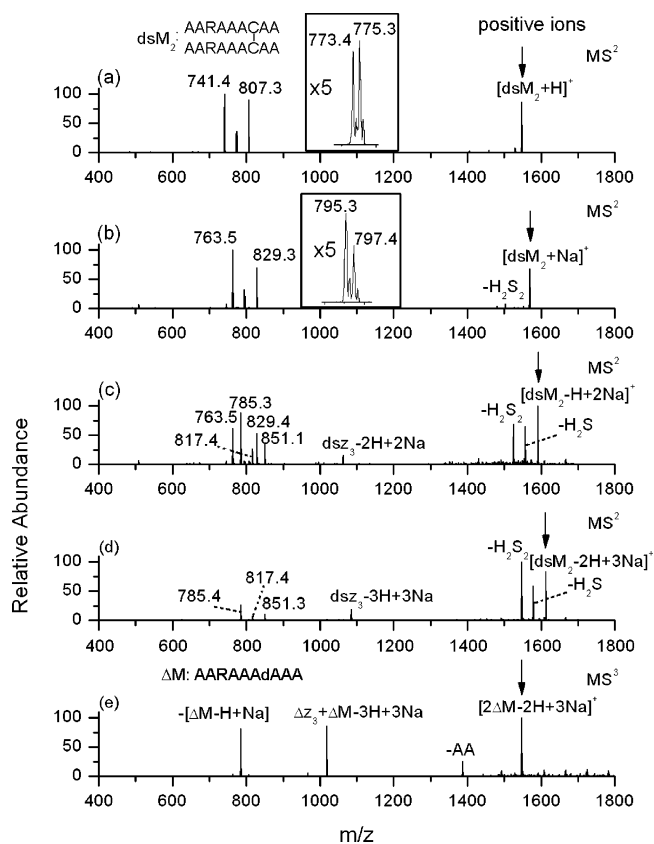
Figure 4. CID spectra of (a) protonated and (b) monosodiated intermolecular disulfide linked AARAAACAA dimer showing products from S–S and S–C bond cleavages. (c) CID spectrum of disodiated disulfide linked AARAAACAA dimer showing products from elimination of H_2S_2 and H_2S along with products from the disulfide bond cleavages. (d) CID spectrum of trisodiated disulfide linked AARAAACAA dimer showing major products from elimination of H_2S_2 and H_2S with some minor products from disulfide bond and backbone cleavages. (e) MS^3 spectrum of the product from elimination of H_2S_2 in (d). Arrows indicate the ion peaks being isolated and collisionally activated.
