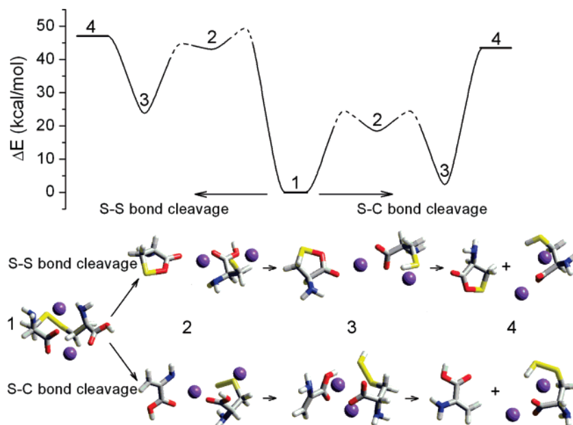
Figure 10. Reaction coordinate diagrams showing relative energies in kcal/mol for S–S bond cleavage (left side) and S–C bond cleavage (right side) of disociated cystine cation at the B3LYP/6-311G** level, including zero-point correction obtained at the same scaled level. Barrier heights are not known. Optimized geometries for corresponding states are obtained at the same scaled level. The reaction mechanism of each numbered step is shown in Scheme 1.
