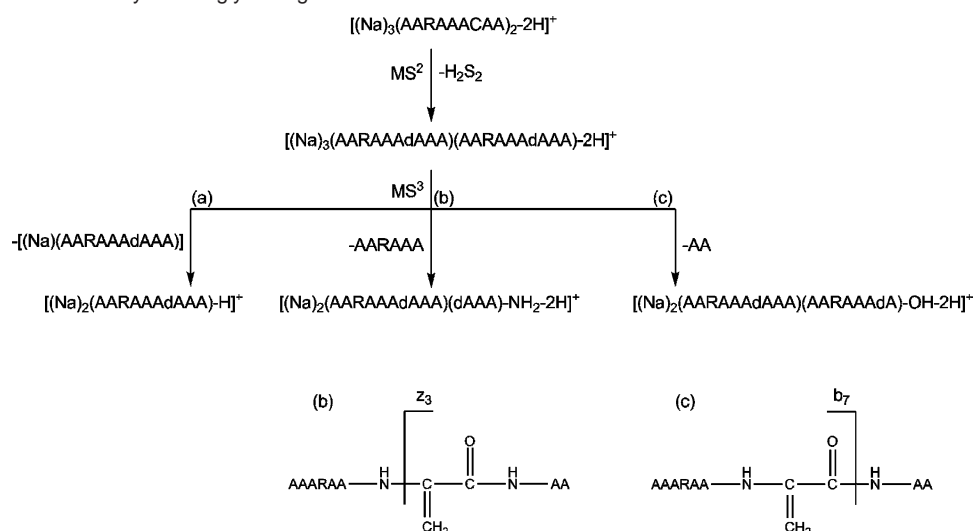
Scheme 2. Dissociation Pathways of Singly Charged Trisodiated MP2 Cation Inferred from CID. Indicated Product Probed by MS 3 a
