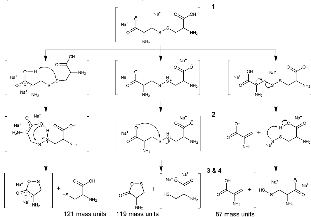
Scheme 1. Proposed Dissociation Mechanisms of Disodiated Cystine Cation via CID a
