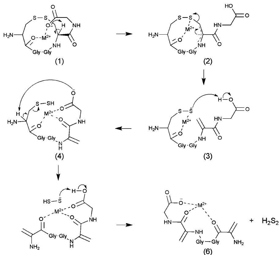
Scheme 5. Proposed \text{H}_2\text{S}_2 Elimination Mechanisms of Singly Charged Cationic Divalent Metal ( \text{M}^{2+} ) Bound Peptide CGGCG with Intramolecular Disulfide Bond a
