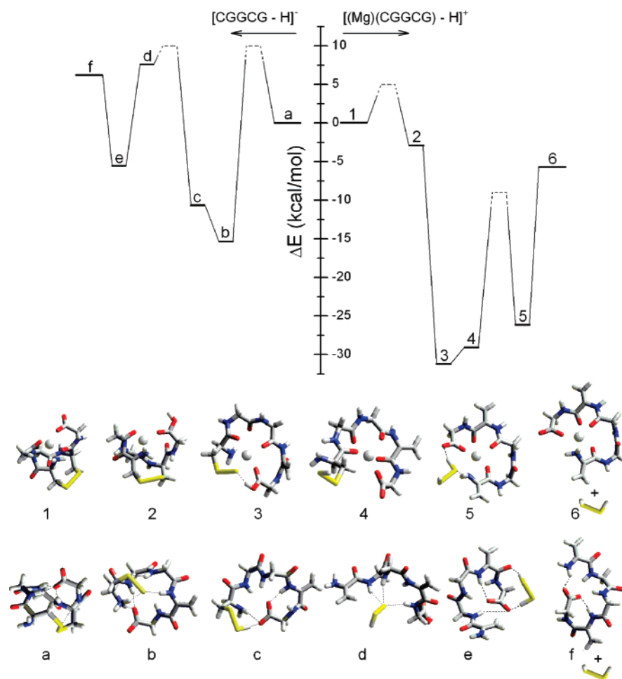
Figure 11. Reaction coordinate diagrams showing relative energies in kcal/mol for the elimination of \text{H}_2\text{S}_2 from deprotonated anionic CGGCG (left side) and magnesium bound cationic CGGCG (right side) at the B3LYP/LACVP level, including zero-point correction obtained at the same scaled level. Barrier heights are not known. Optimized geometries are obtained at the same scaled level. The geometries for reactants, products, and intermediates are shown below the diagram. The reaction mechanism of each labeled and numbered step is shown in Schemes 4 and 5, respectively.
